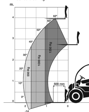
(*) Standard carriage with side-shift
