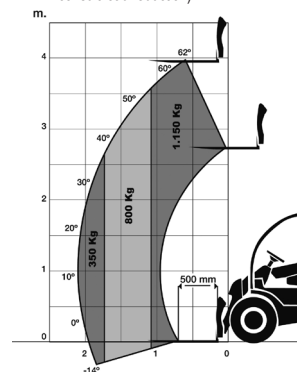
(**) Universal / Euro 8 carriage (with side-shift consult load reduction)
